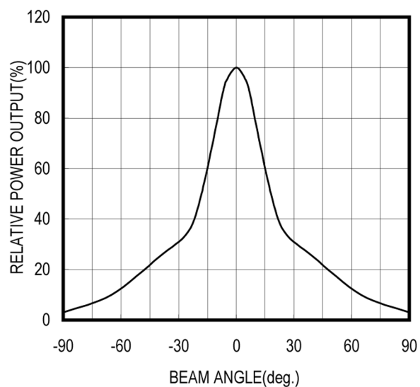
RADIATION PATTERN
