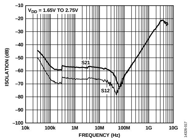
Figure 7. Isolation vs. Frequency over Supplies (RFx to RFC)
