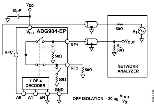
Figure 17. Off Isolation
