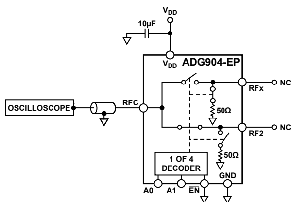
Figure 20. Video Feedthrough
