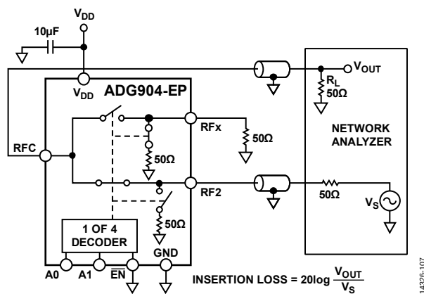
Figure 18. Insertion Loss
