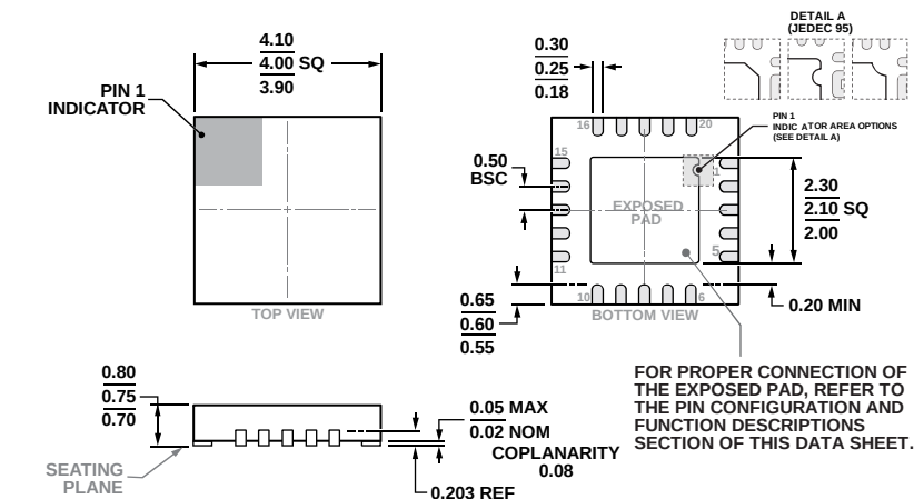
Figure 23. 20-Lead Lead Frame Chip Scale Package [LFCSP] 4 mm × 4 mm Body and 0.75 mm Package Height (CP-20-6) Dimensions shown in millimeters
