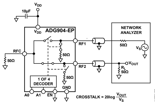
Figure 19. Crosstalk
