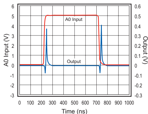
Figure 21. A0 Switching Glitch
