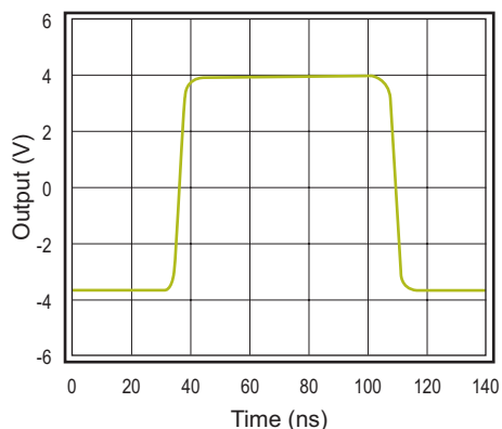
Figure 19. Pulse Response
