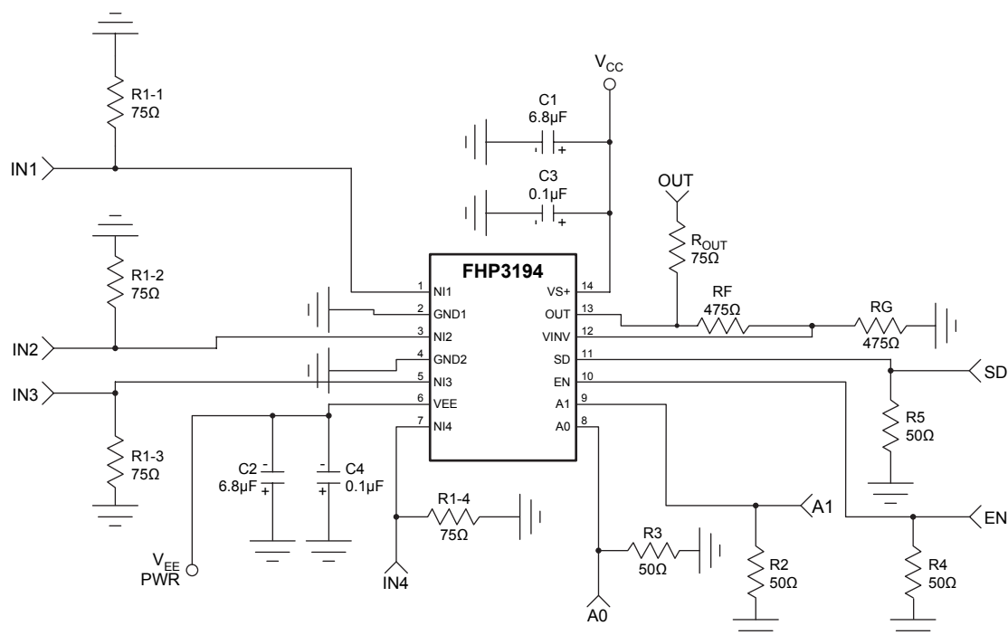
Figure 40. FHP3194 Schematic Diagram
