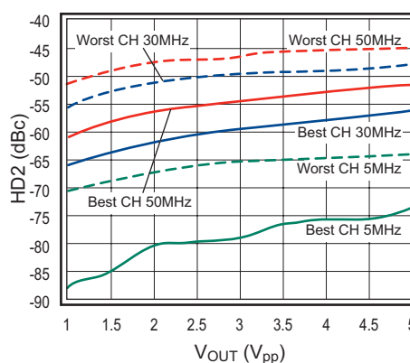
Figure 12. HD2 vs. V_{OUT}
