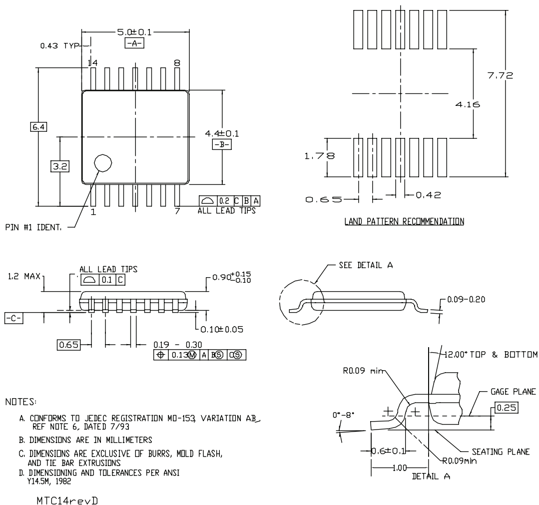
Figure 42. TSSOP-14 Package
