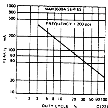
Fig. 12. Max Peak Current vs. Duty Cycle
