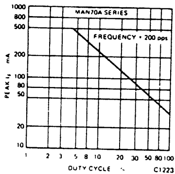
Fig. 15. Max Peak Current vs. Duty Cycle
