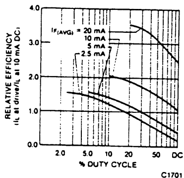
Fig. 11. Relative Efficiency vs. Duty Cycle
