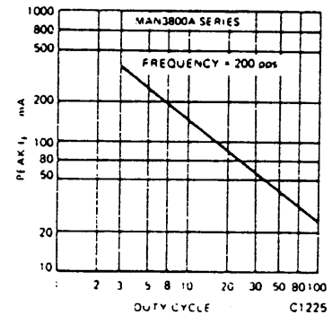
Fig. 16. Max Peak Current vs. Duty Cycle
