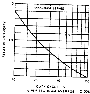
Fig. 17. Luminous Intensity vs. Duty Cycle
