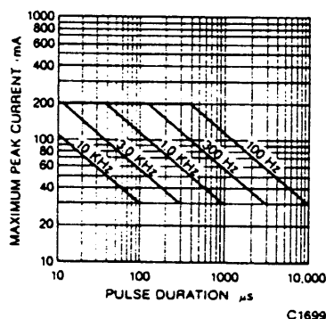
Fig. 10. Maximum Peak Current vs. Pulse Duration
