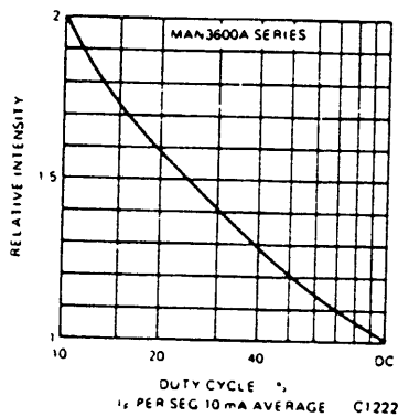
Fig. 13. Luminous Intensity vs. Duty Cycle
