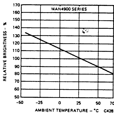
Fig. 5. Relative Luminous Intensity vs. Temperature
