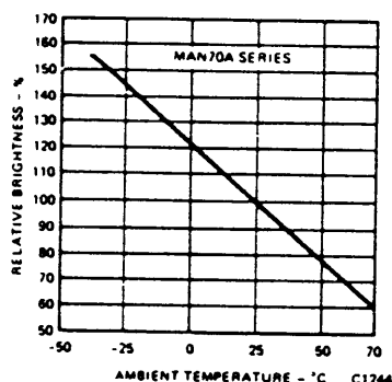
Fig. 7. Relative Luminous Intensity vs. Temperature
