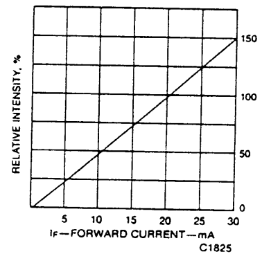
Fig. 18. Relative Luminous Intensity vs. Forward Current
