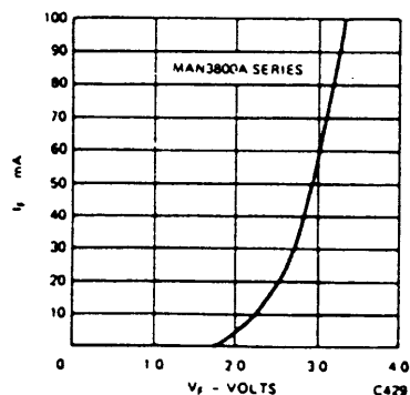
Fig. 8. Forward Current vs. Forward Voltage
