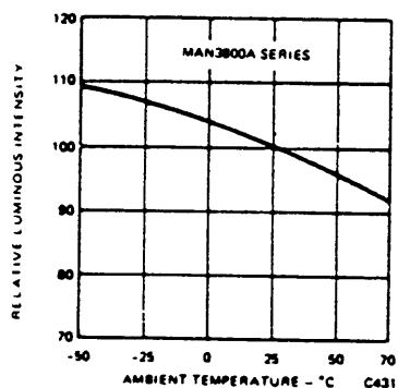
Fig. 9. Relative Luminous Intensity vs. Temperature
