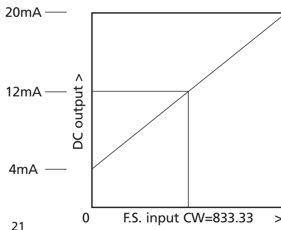
Ex. 2 20KW input, 4 to 20mA output
