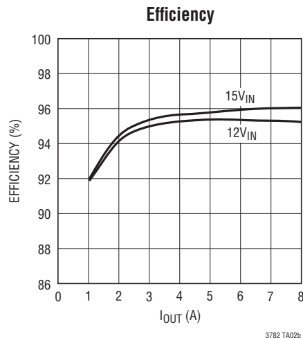
3782 TA02 L1, L2: PULSE PB2020-103 ALL CERAMIC CAPACITORS ARE X7R, TDK *OUTPUT CURRENT WITH BOTH INPUTS PRESENT
