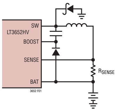
Figure 1. Programming Maximum Charge Current Using R_{SENSE}
