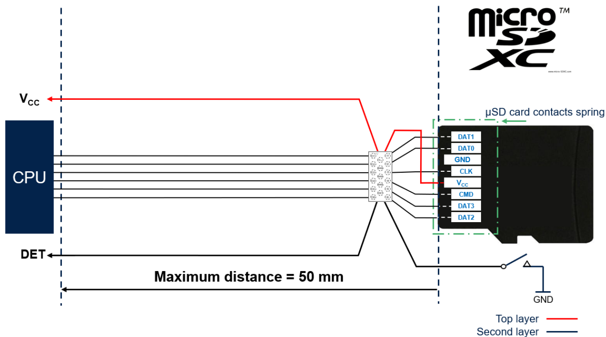
Figure 12. Layout recommendation
