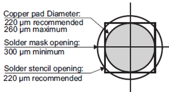
Figure 14. Footprint recommendations
