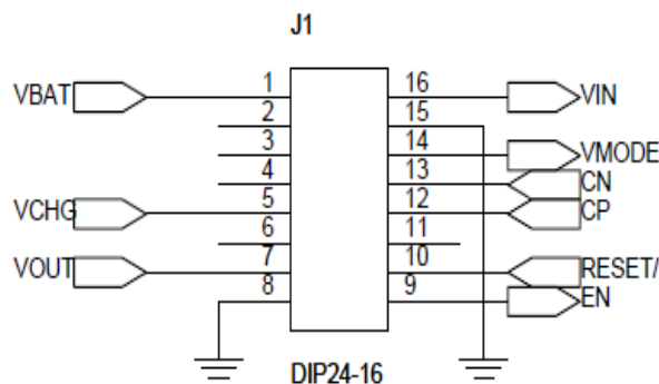
Figure 12: CBC3105-R4C Eval Board Pin-out
