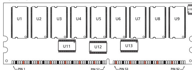
Figure 2: Pin Locations
