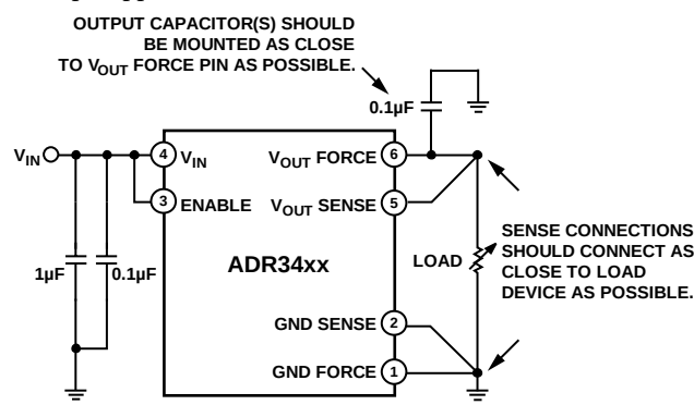
Figure 41. Application Showing Kelvin Connection
