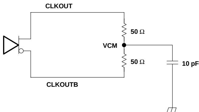
Figure 1. Test Load and Voltage Definitions ( V_{\text{O(STOP)}} , V_{\text{OX}} , V_{\text{OH}} , V_{\text{OL}} )
