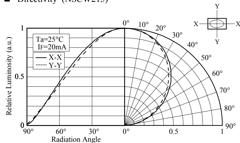
■ Directivity (NSCW215)
