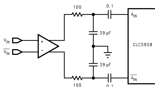
Figure 24. Differential Amplifier
