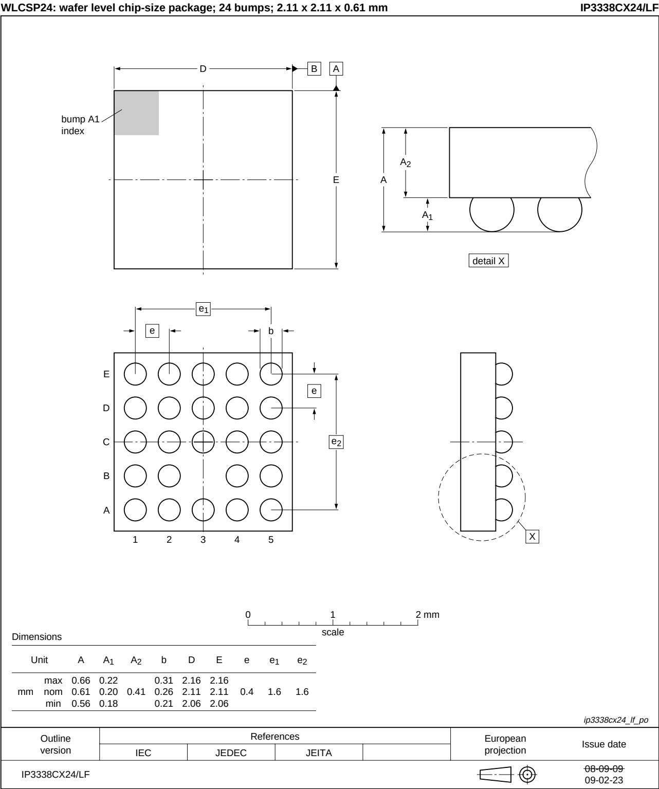
Fig 7. Package outline IP3338CX24/LF (WLCSP24)
