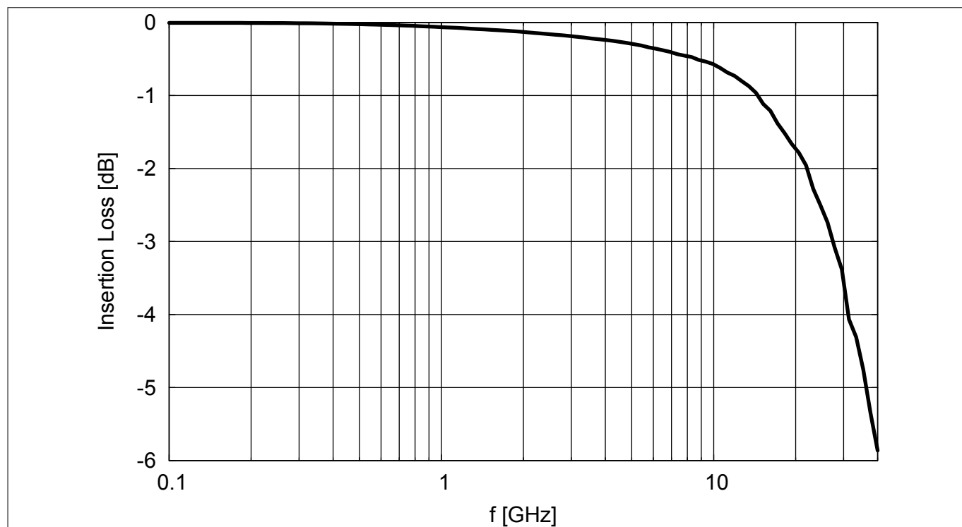
Figure 12 Insertion loss vs. frequency in a 50 \Omega system
