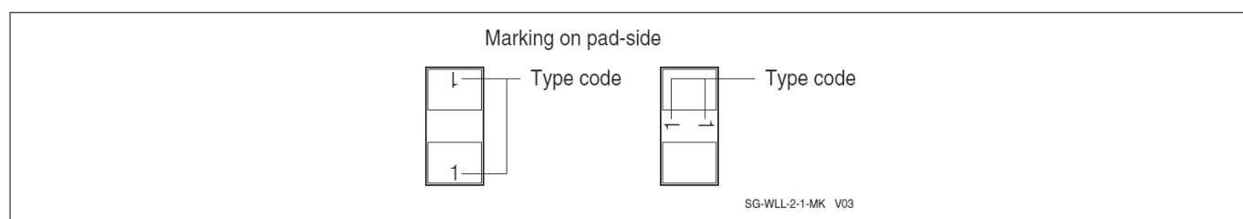
Figure 16 WLL-2-1 marking example (see Device information )
