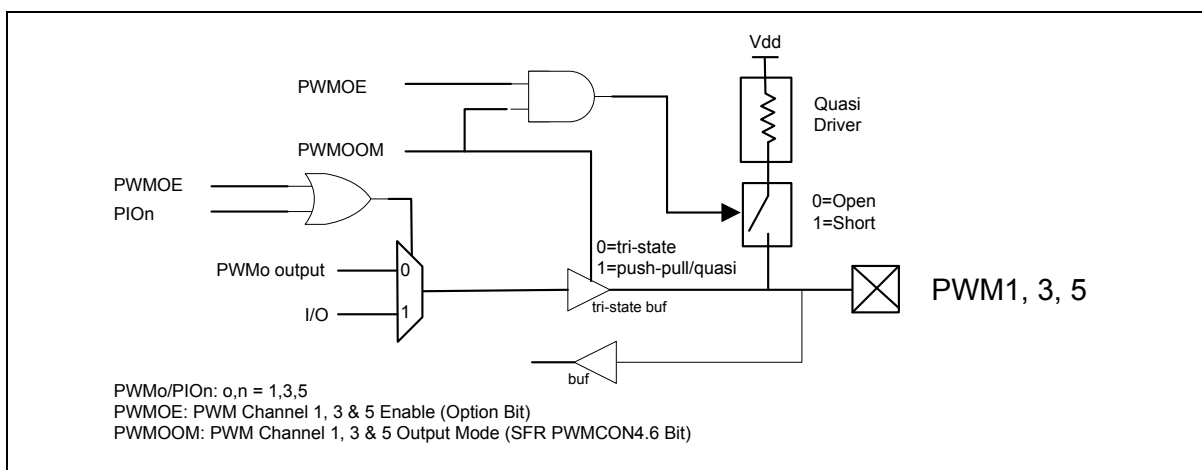
Figure 14-4: PWM1, 3 & 5 I/O pins
