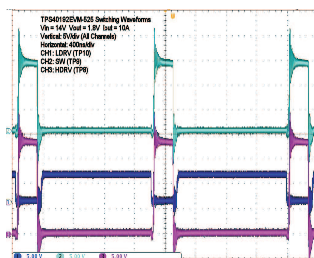
Figure 22. Switching Waveforms
