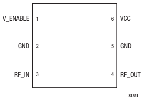
Figure 1. SKY65404-11 Pinout – 6-Pin QFN Package (Top View)
