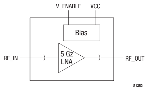
Figure 2. SKY65404-11 LNA Block Diagram
