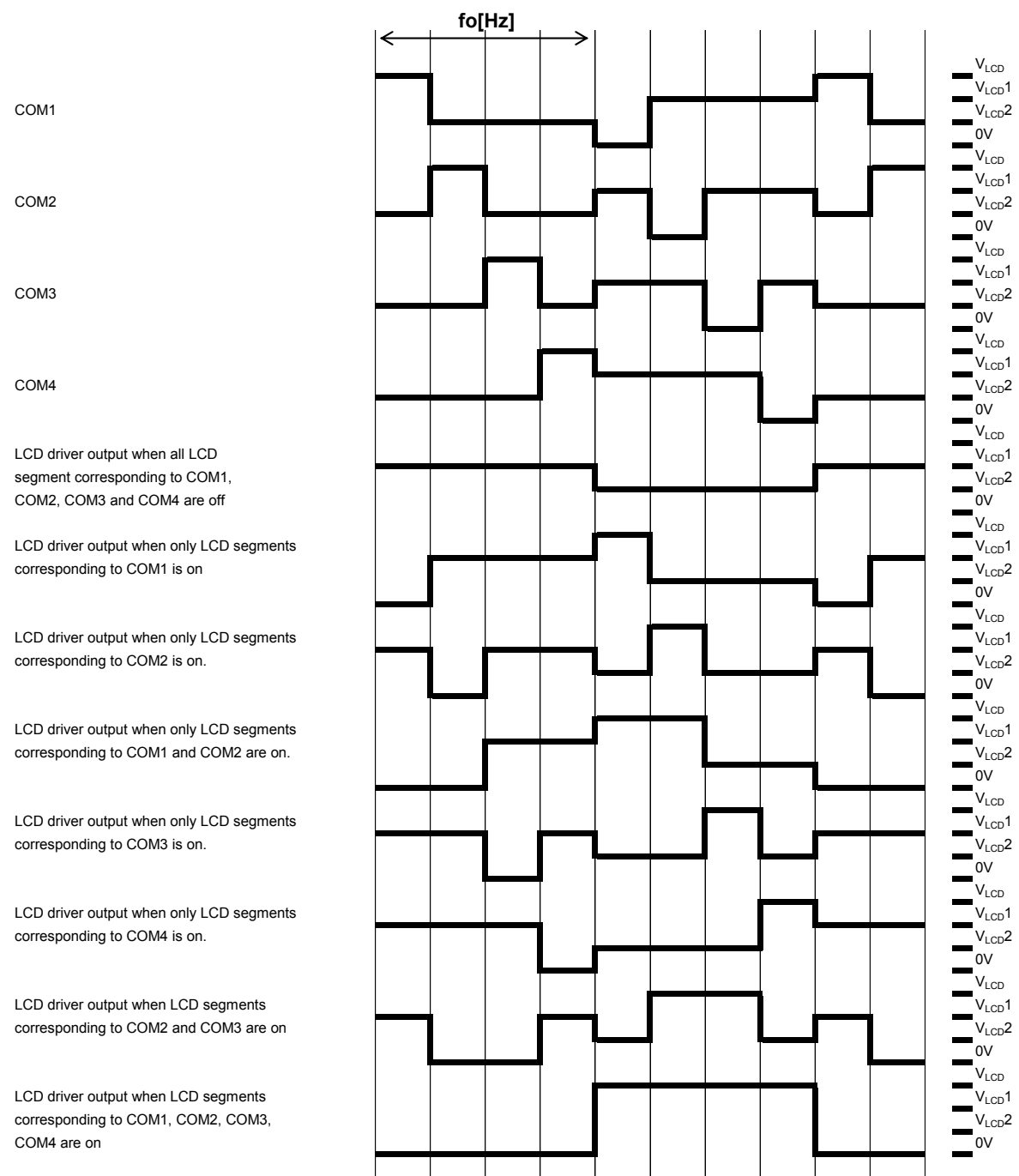
Figure 33. LCD Waveform (Frame Inversion, 1/4 DUTY, 1/3BIAS)
