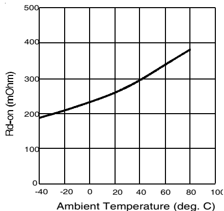
Figure 4. Typical On-Resistance
