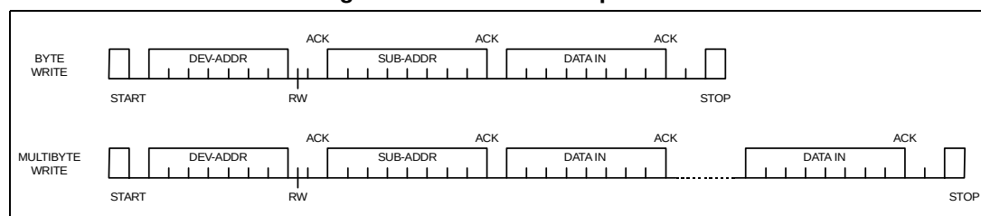
Figure 9. Write-mode sequence
