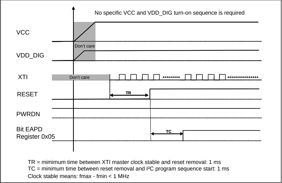
Figure 3. Power-on sequence
