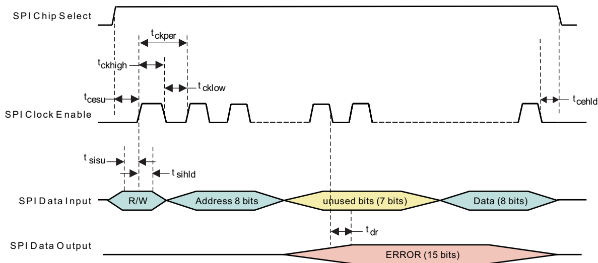
Figure 6-3. SPI Interface Timing
