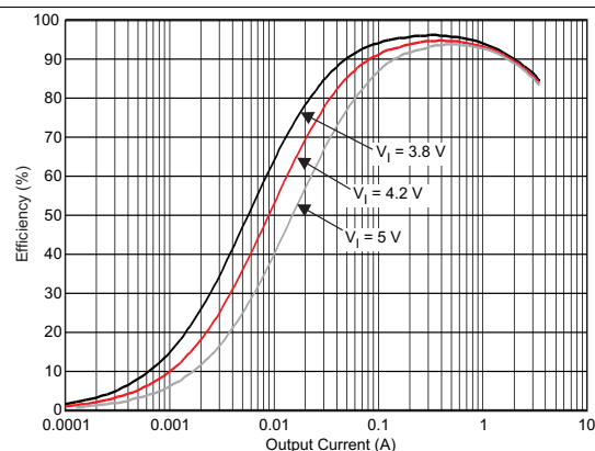
DCDC4 V_O = 3.3 V DEF322512-1 \mu H PWM Mode 25°C
