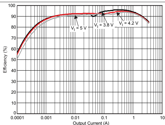
DCDC4 V_O = 3.3 V DEF322512-1 \mu H PFM Mode 25°C
