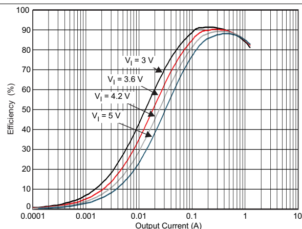
DCDC2 V_O = 1.8 V LQM2NPN-1 \mu H PWM Mode 25°C
