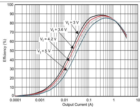
DCDC4 V_O = 1.1375 V DEF322512-1 \mu H PWM Mode 25°C
