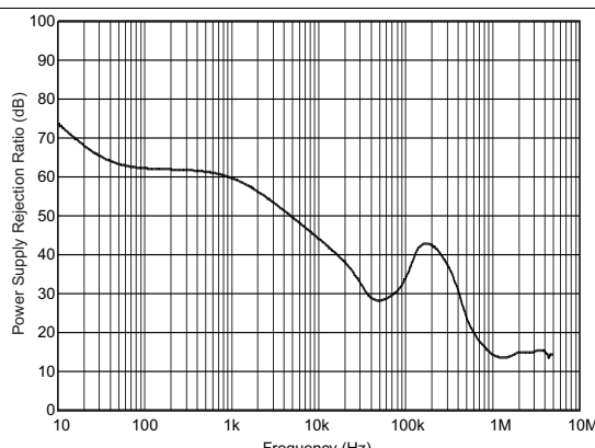
V_{IN\_LDO} = 3.2 V I_{OUT} = 225 mA V_{OUT} = 2.7 V
