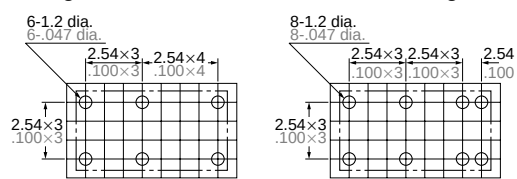
PC board pattern (Copper-side view) Single side stable 2 coil latching
