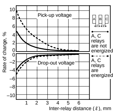
6.-(2) Influence of adjacent mounting (1a1b type)
