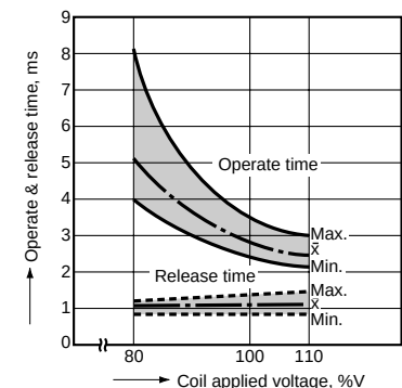
4.-(2) Operate & release time (without diode, 1a1b type)
