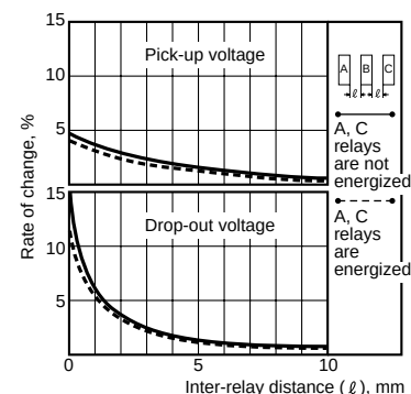
6.-(3) Influence of adjacent mounting (2a type)
