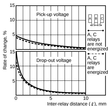
6.-(1) Influence of adjacent mounting (1a type)
