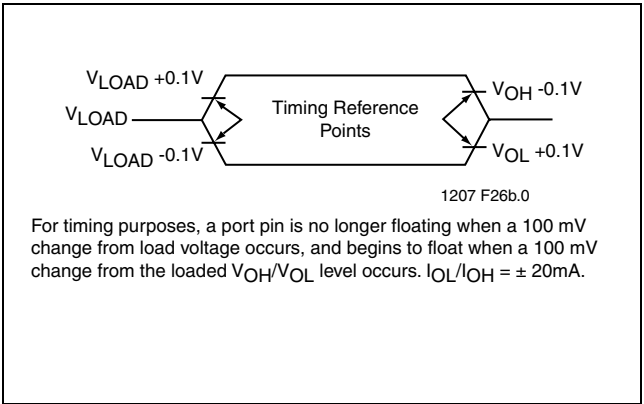
FIGURE 13-9: FLOAT WAVEFORM
