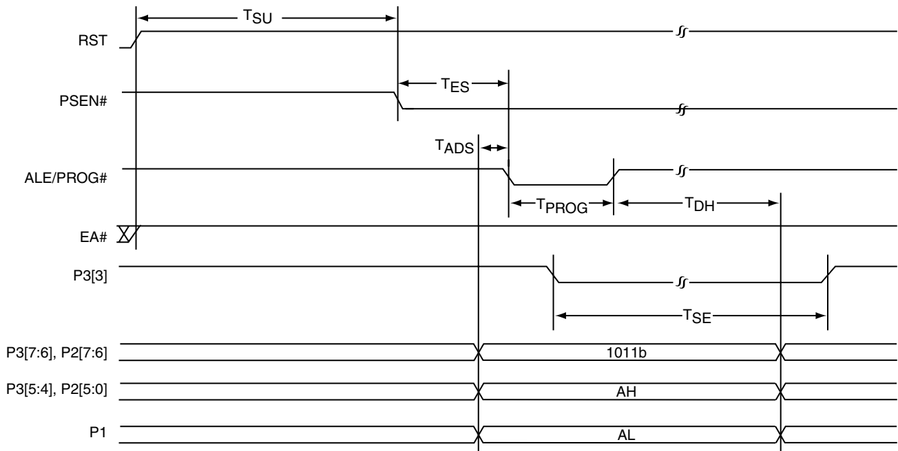
FIGURE 13-19: SECTOR-ERASE
