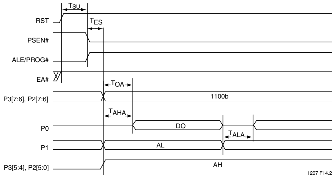
FIGURE 13-23: BYTE-VERIFY
