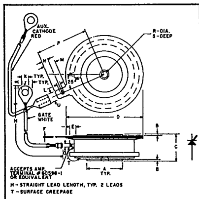
C380__X500 Outline Drawing
