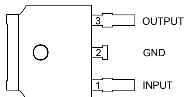
(TO-252-2 (3)) (Option 1)
