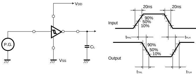
Fig.2 Switching characteristics measurement circuit
