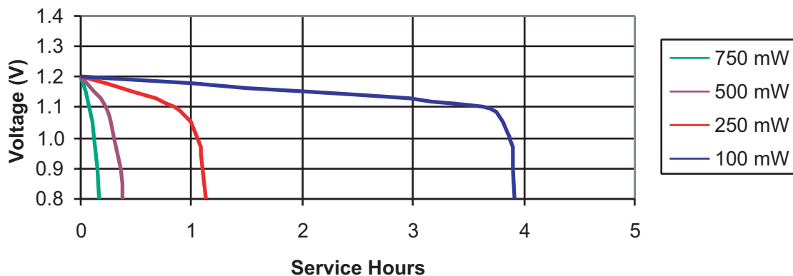
Discharge Characteristics at Various Power Drains
