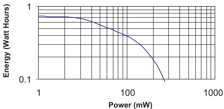
Delivered Energy vs Power Drain @20° C to 1.0 Volts
