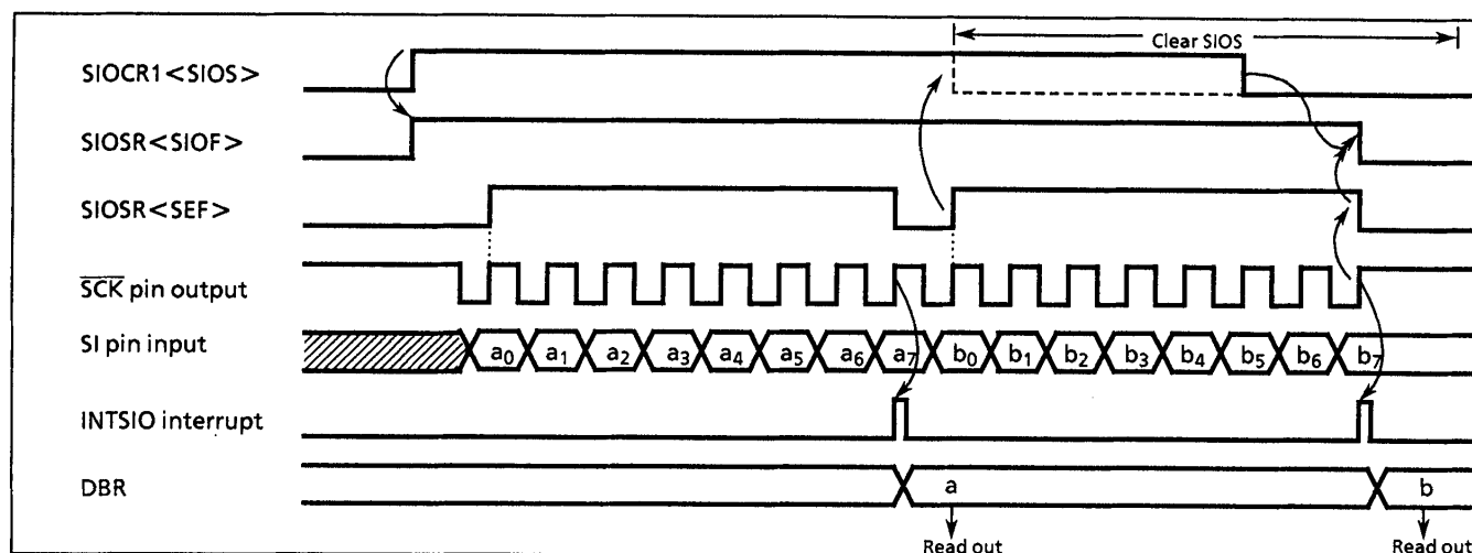
Figure 2-55. Receive Mode (Example: 8-bit, 1 word, internal clock)
