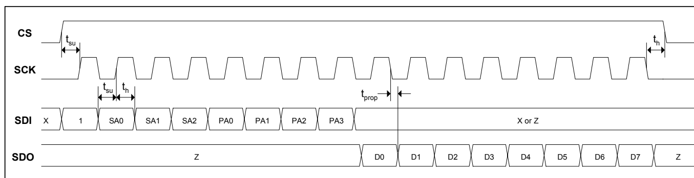
Figure 6: Read Operation
