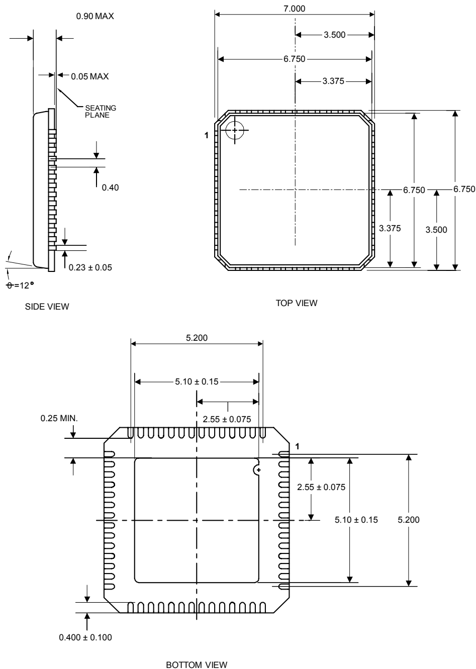
56-pin Quad Flat No-lead package (QFN) (All dimensions in mm)
