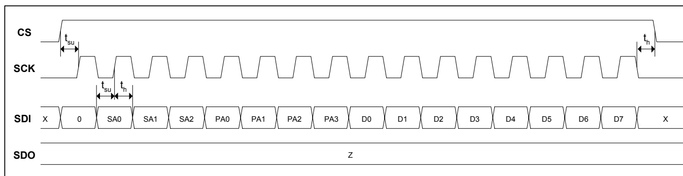
Figure 7: Write Operation
