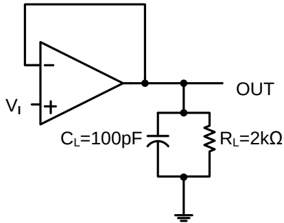
Figure 1. Unity-Gain Amplifier
