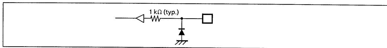
Figure 1-2. TEST pin
