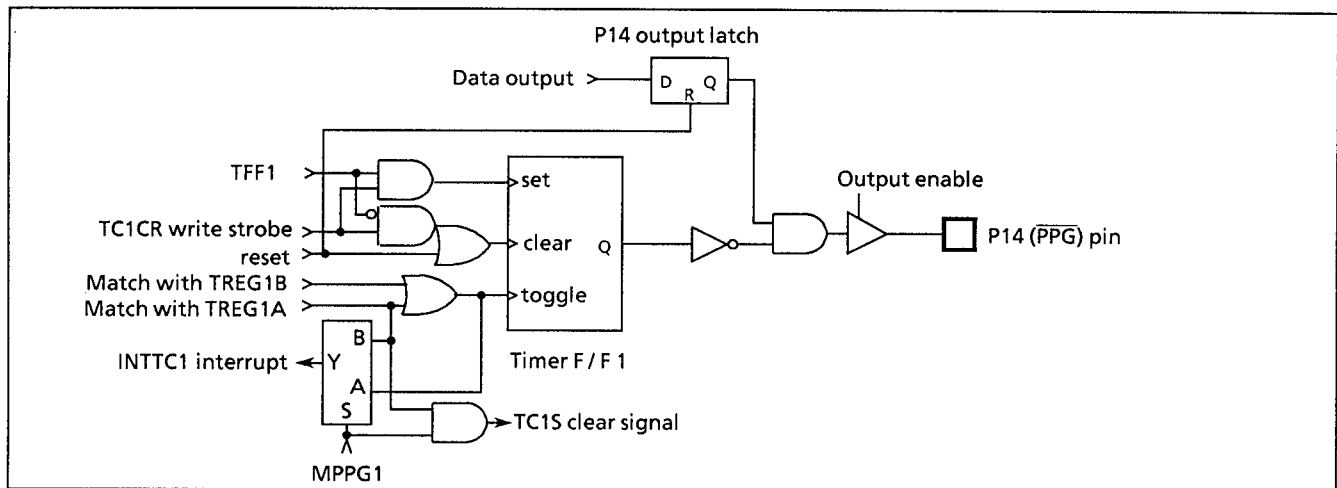
Figure 2-20. \overline{\text{PPG}} Output
