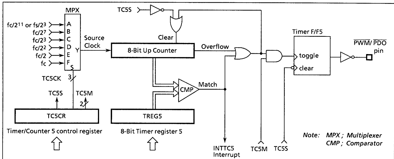
Figure 2-28. Timer/Counter 5 (TC5)
