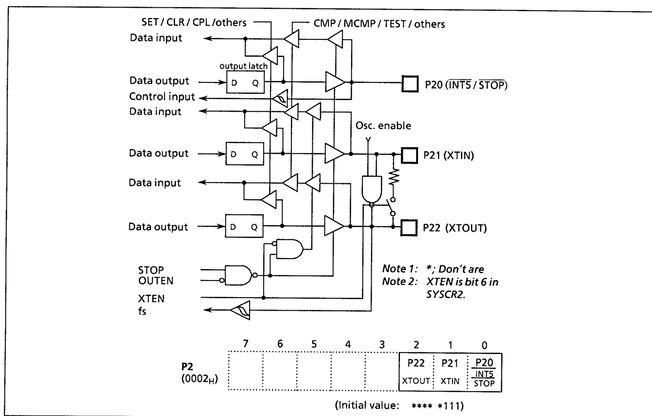
Figure 2-4. Port P2
