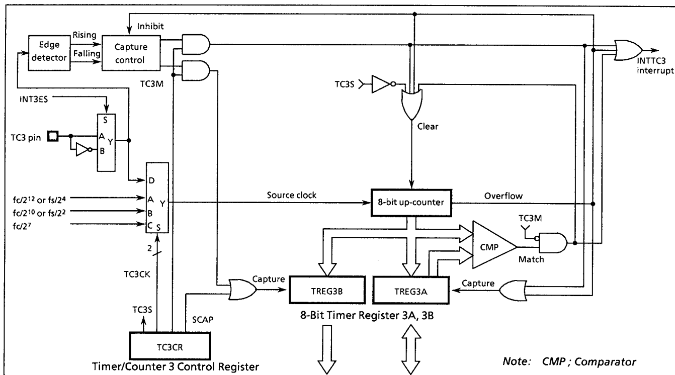
Figure 2-25. Timer/Counter 3
