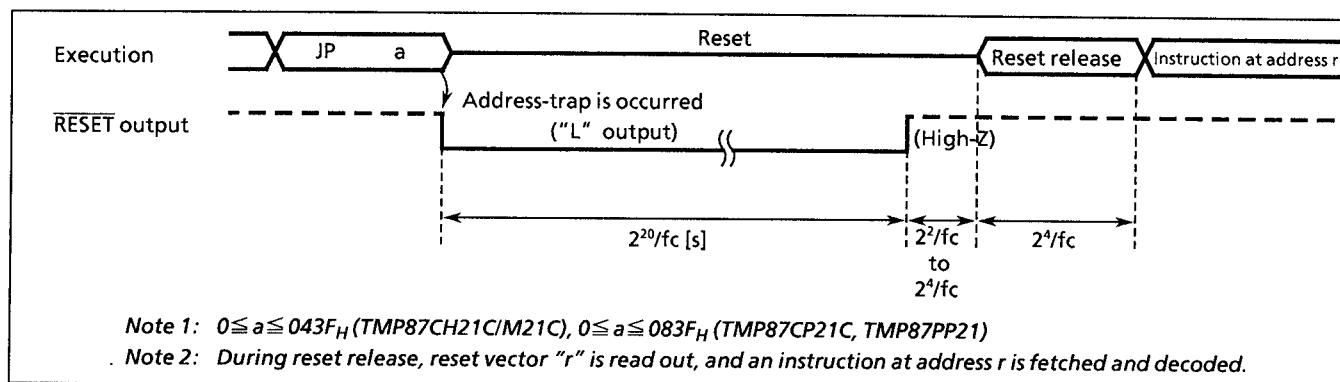
Figure 1-31. Address-Trap-Reset
