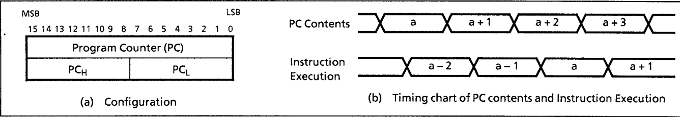
Figure 1-3. Program Counter
