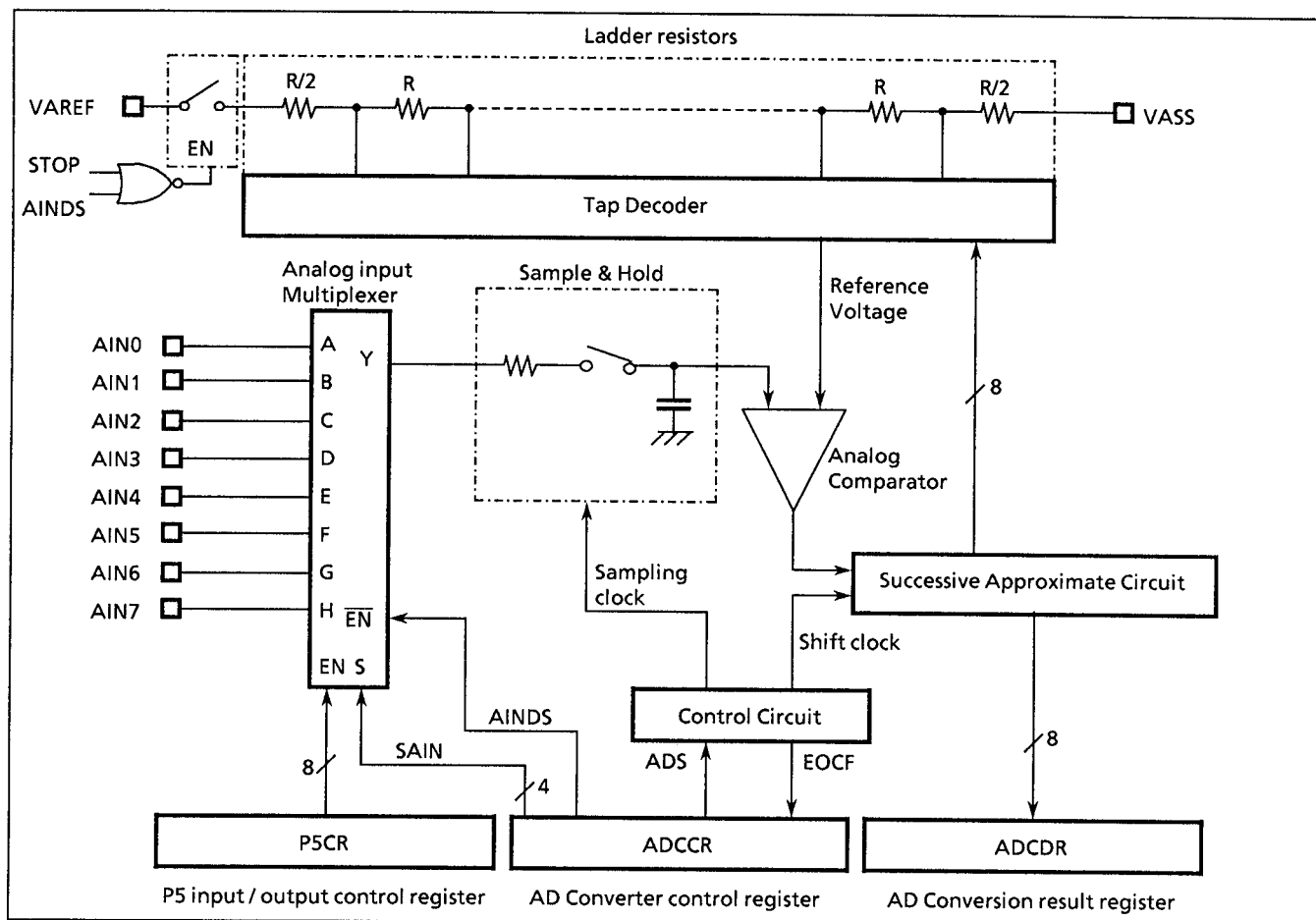
Figure 2-42. AD Converter
