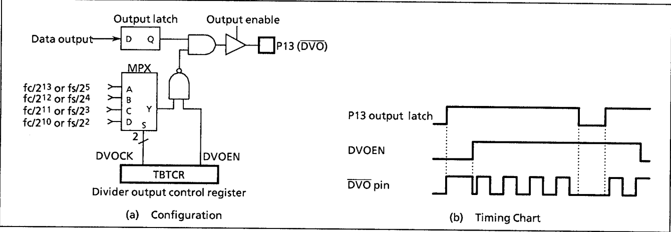
Figure 2-12. Divider Output
