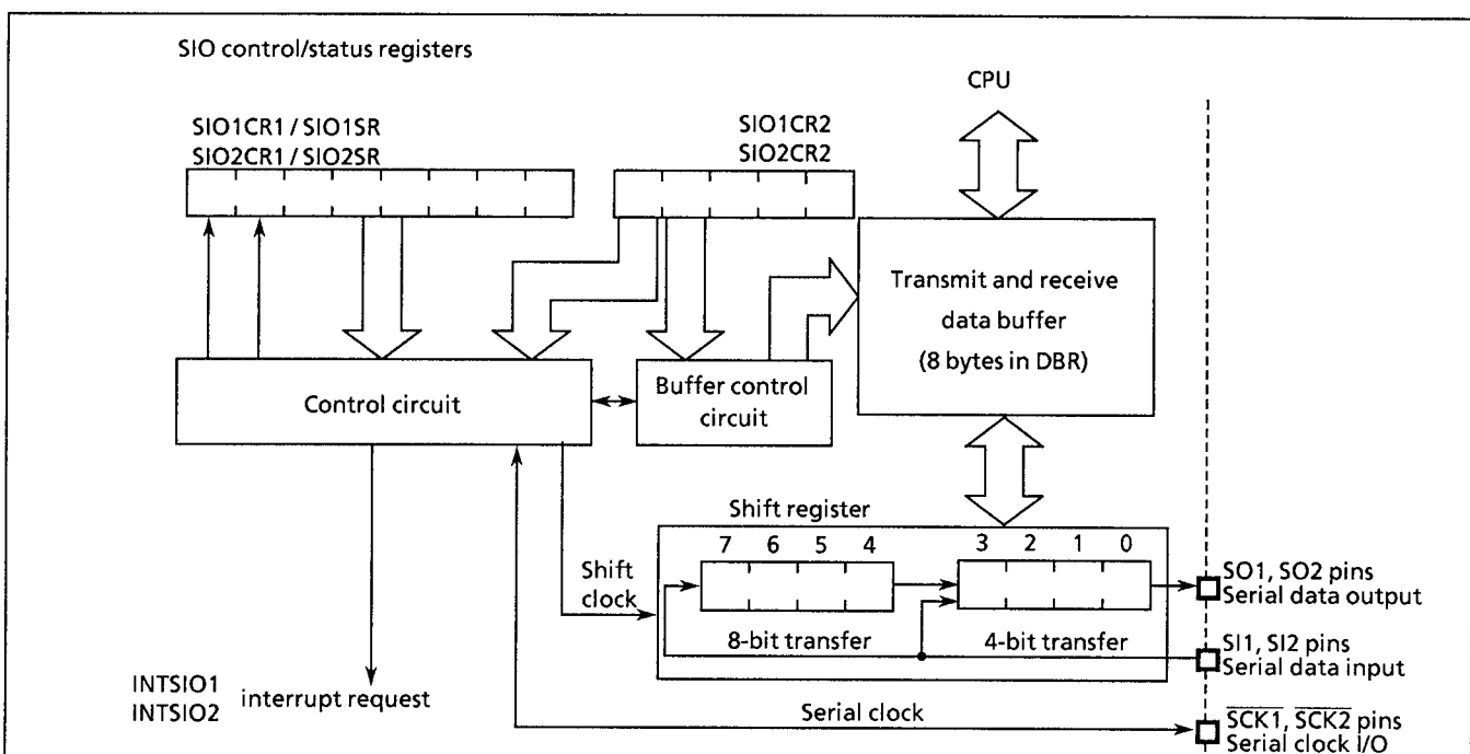
Figure 2-32. Serial Interfaces
