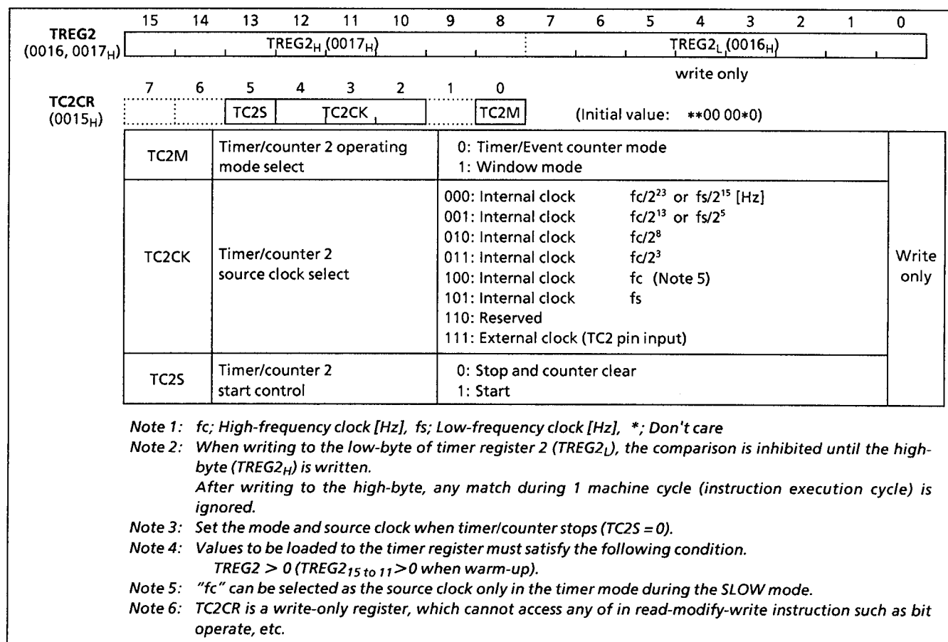
Figure 2-23. Timer Register 2 and TC2 Control Register
