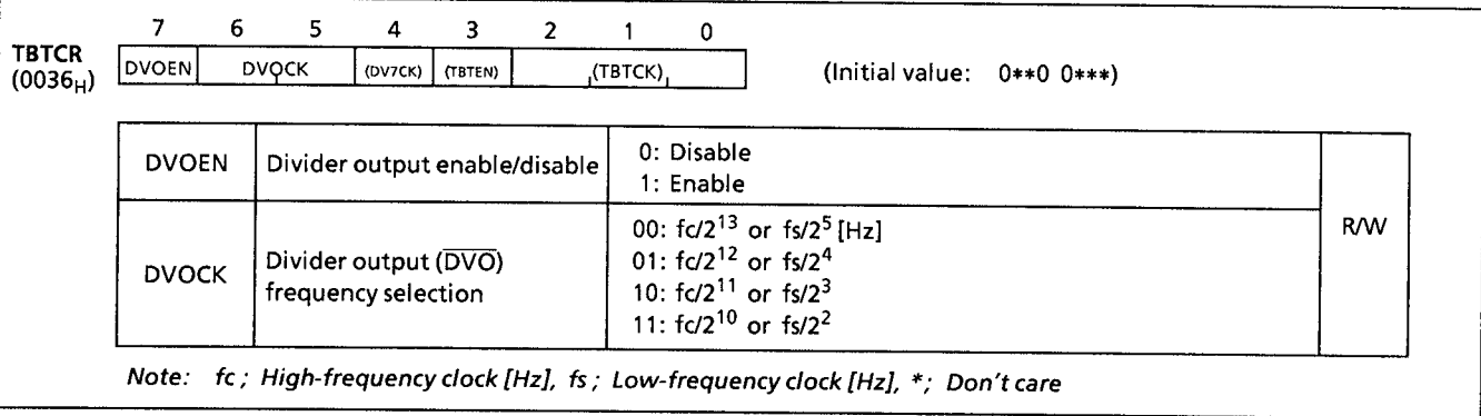
Figure 2-11. Divider Output Control Register
