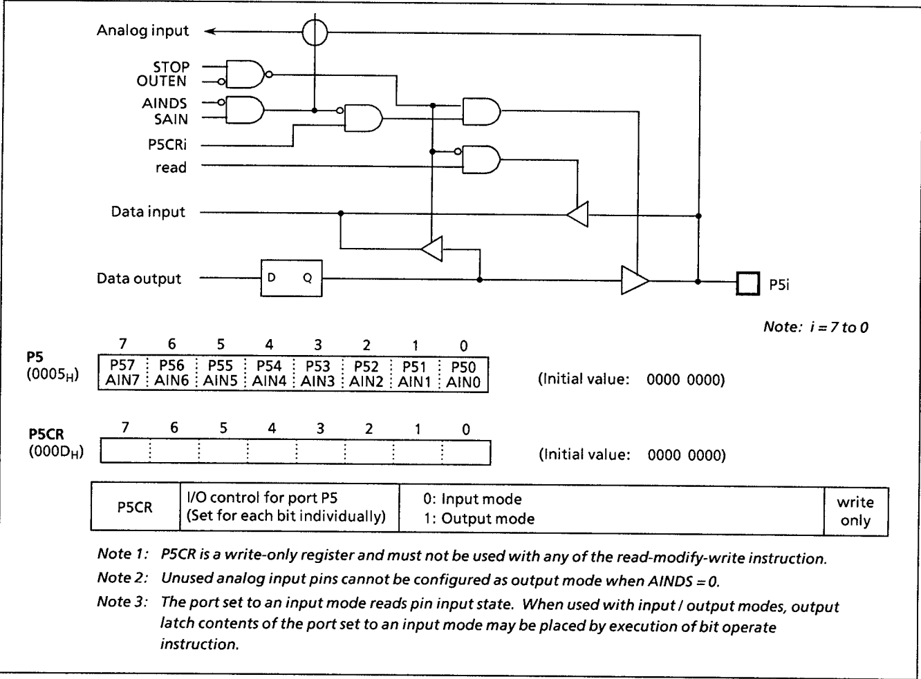
Figure 2-7. Port P5
