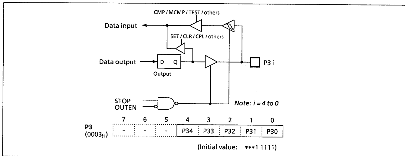
Figure 2-5. Port P3
