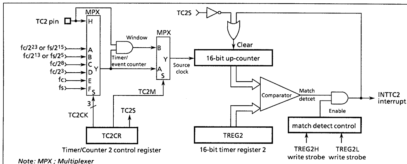
Figure 2-22. Timer/Counter 2 (TC2)
