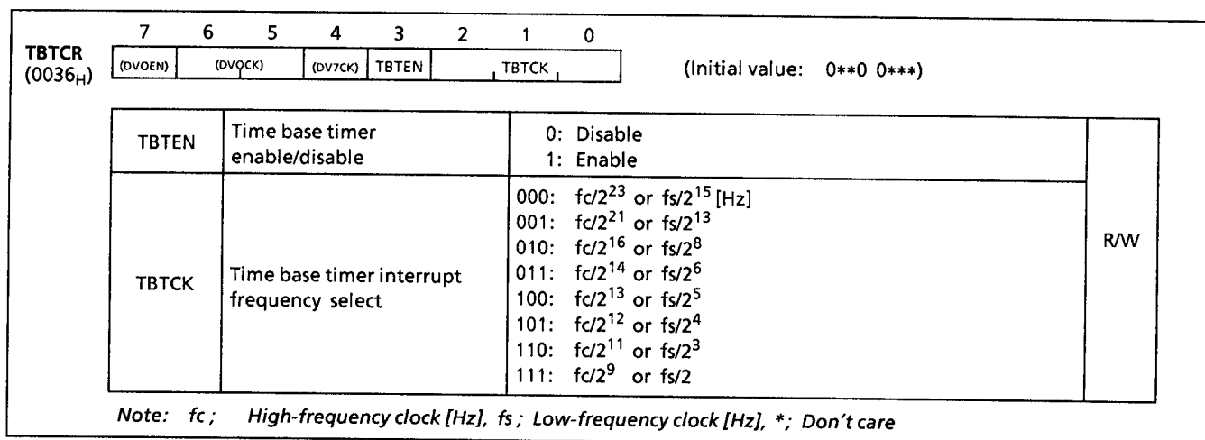
Figure 2-10. Time Base Timer and Divider Output Control Register
