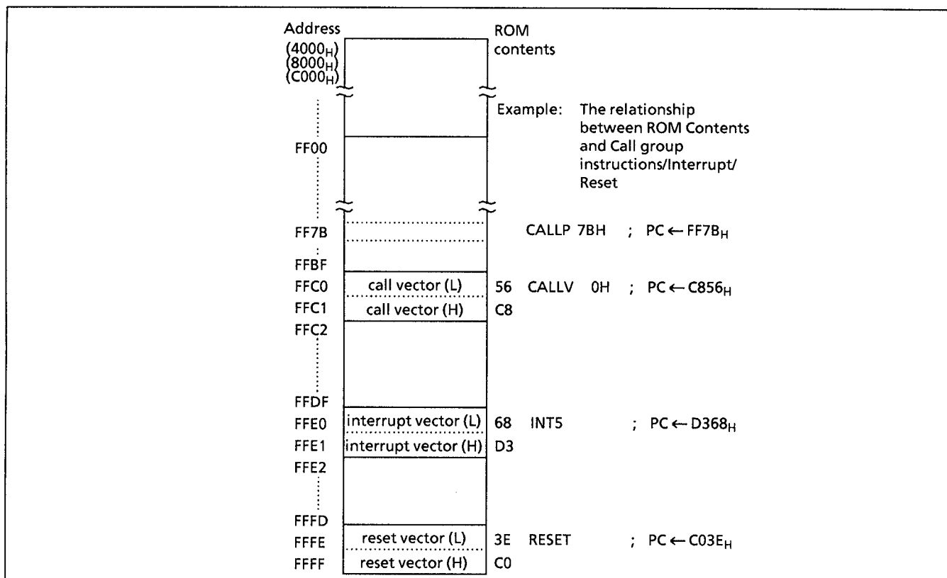
Figure 1-2. Program Memory Map
