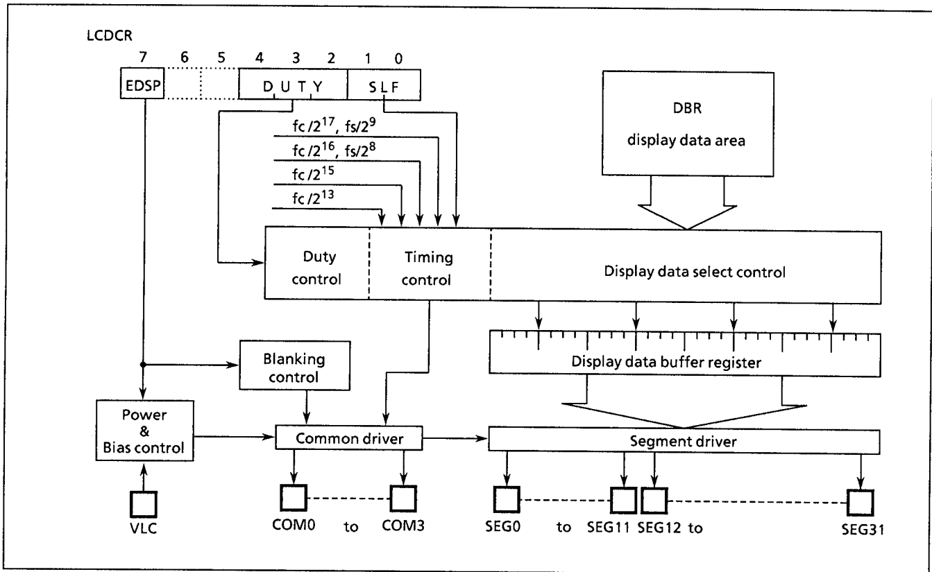
Figure 2-47. LCD driver
