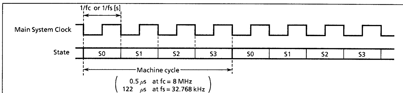
Figure 1-13. Machine Cycle
