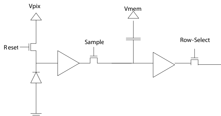
Figure 6. 6T Pixel Architecture
