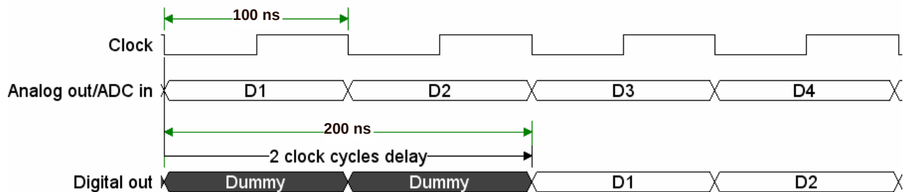
Figure 8. ADC Timing
