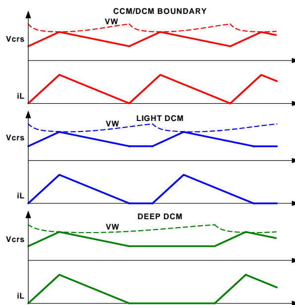
FIGURE 9. PERIOD STRETCHING
