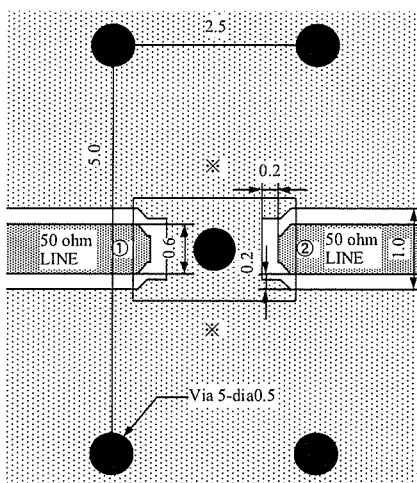
Electrodes pattern
