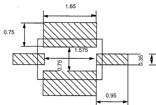
Resist pattern (aperture size)
