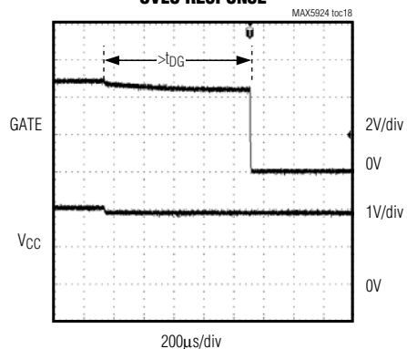
UVLO RESPONSE
