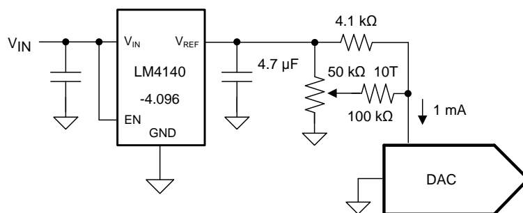
Figure 27. Precision DAC Reference Schematic
