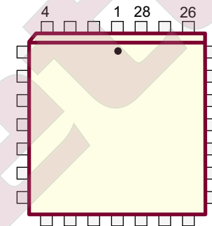
28-Lead PLCC (PJ)
