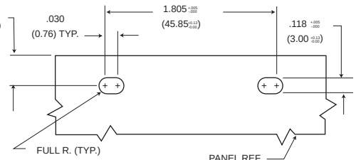
Figure 3 Edgeboard Mounting
