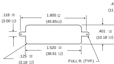
Figure 2 Rear Mounting
