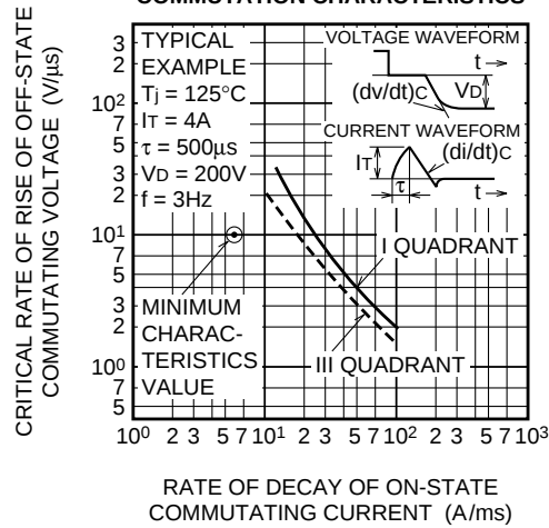
COMMUTATION CHARACTERISTICS
