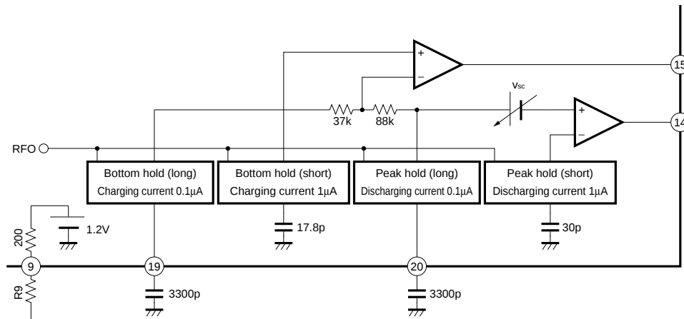
Fig.7 DET block
