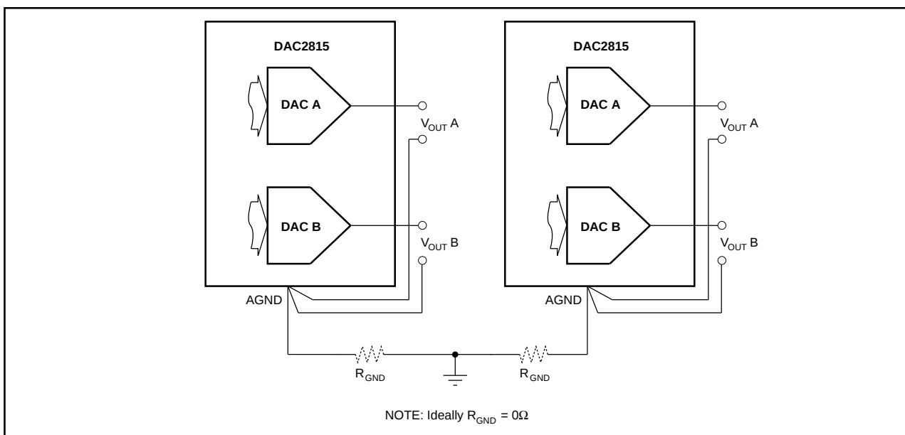
FIGURE 2. Recommended Ground Connections for Multiple DAC packages.
