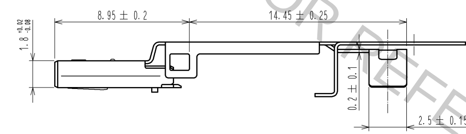
Fig-2 COMPONENT BREAK OFF FIGURE (FREE)
