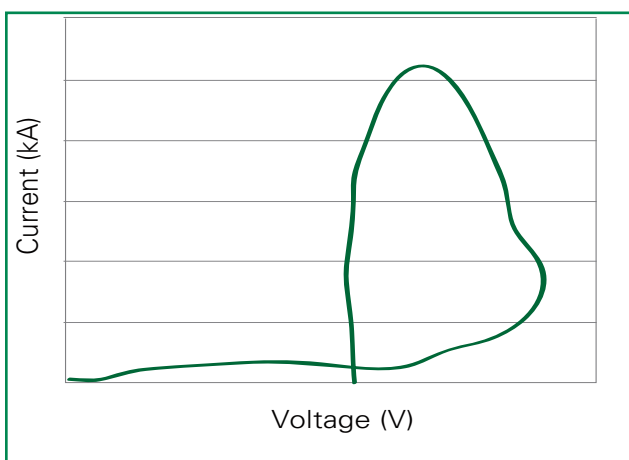
Figure 4 - Surge Response
