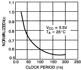
NORMALIZED SUPPLY CURRENT vs. CYCLE PERIOD
