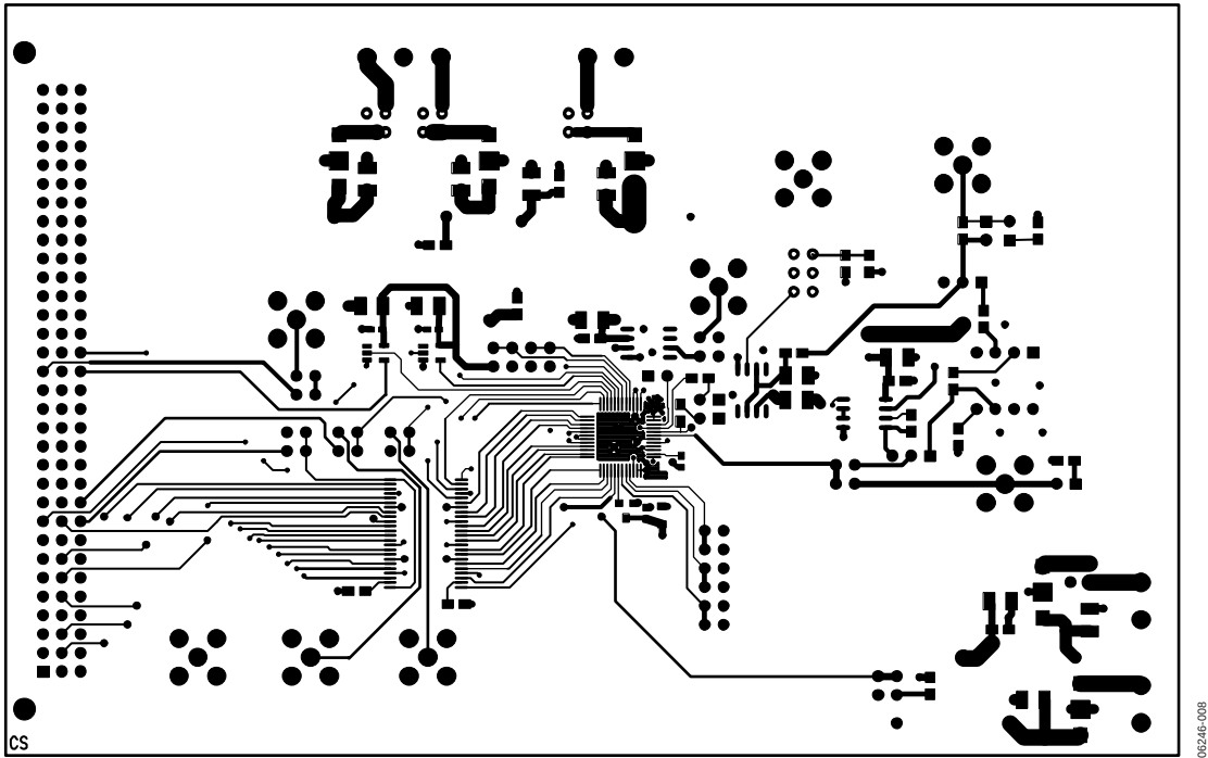
Figure 10. Top Layer Etch
