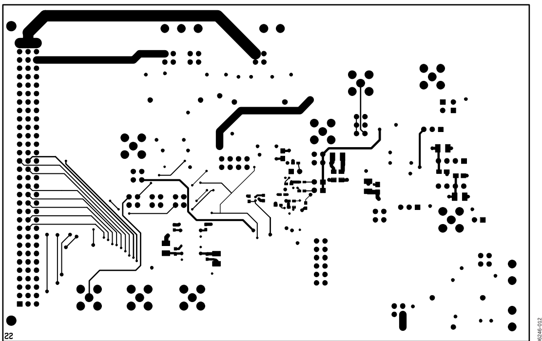
Figure 14. Bottom Layer Etch
