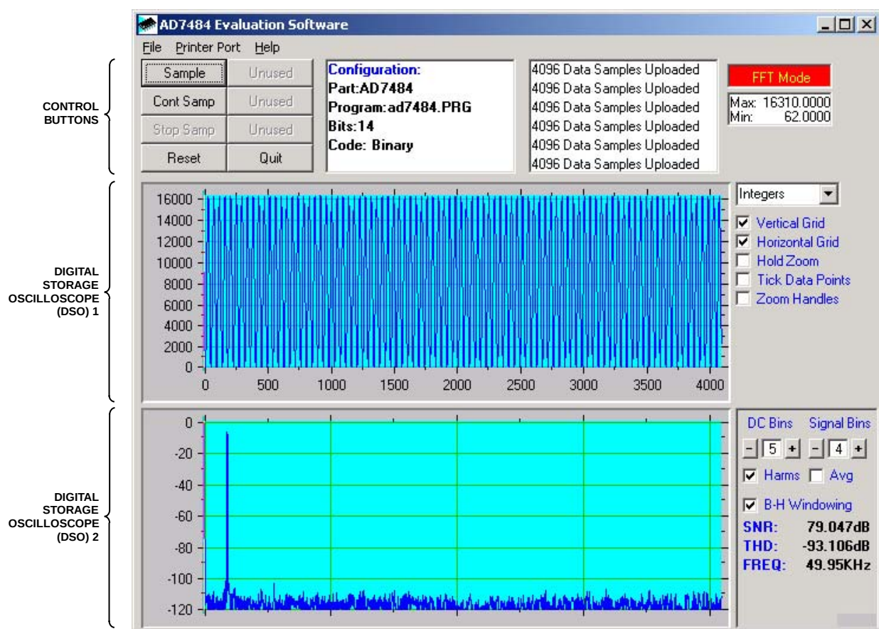
Figure 3. AD7484 Main Window
