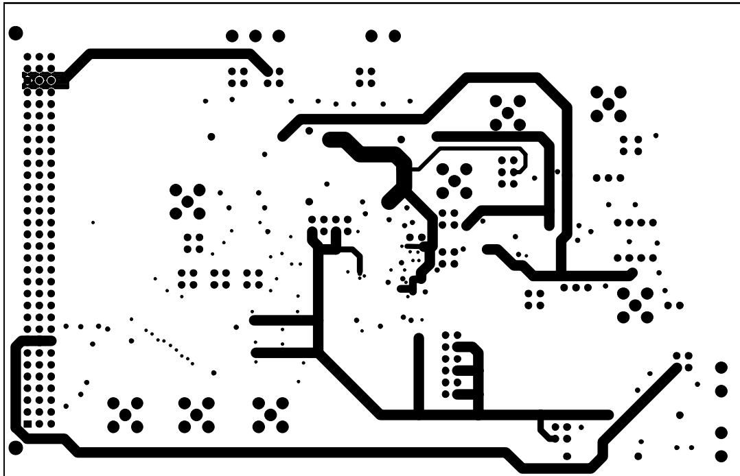
Figure 12. Inner Layer
