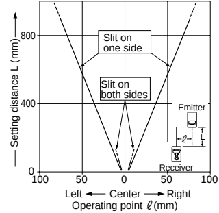
Parallel deviation with rectangular slit masks ( 2 \times 6\text{mm} )
