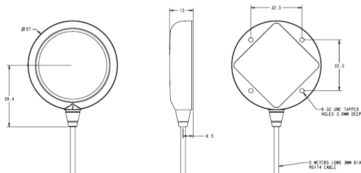
Dimensions (mm) p/n 32-2400-0
