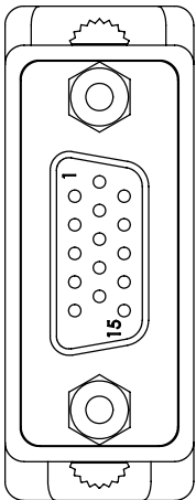
FEMALE 15-PIN HIGH DENSITY D-SUB CONNECTOR
