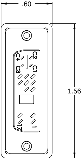
MALE DVI-A CONNECTOR
